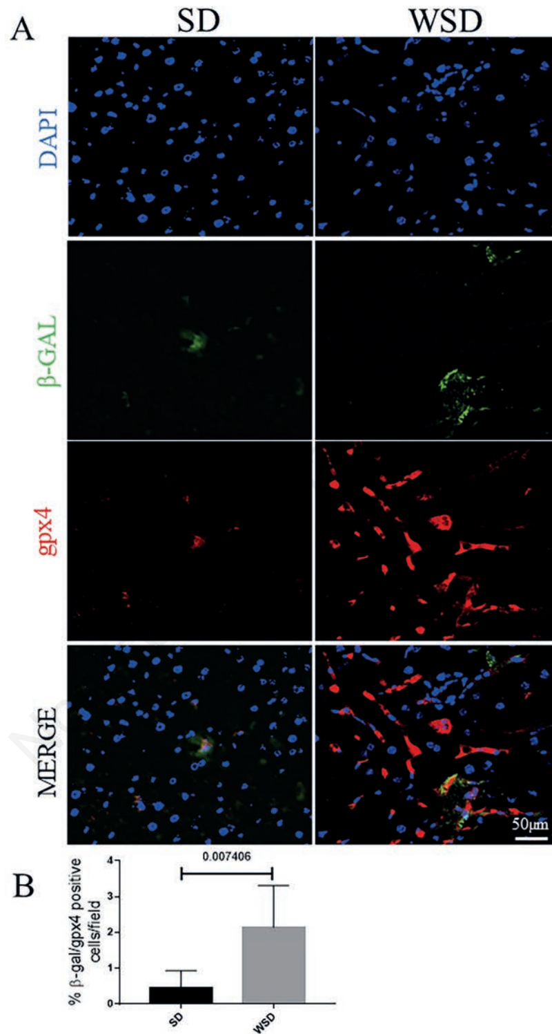
Figure 5. A) Immunofluorescence for \beta -gal (green) and Gpx4 (red) showed an increase in \beta -gal/Gpx4-positive cells in WSD-fed mice compared to the SD group; Nuclei are counterstained with DAPI (blue); original magnification 20 \times , scale bar: 50 \mu m. B) Quantification of A. These images are representative of n=8 SD, and n=8 WSD mice. Data were analyzed using the Mann-Whitney test; SD, standard diet; WSD, Western-style diet.
