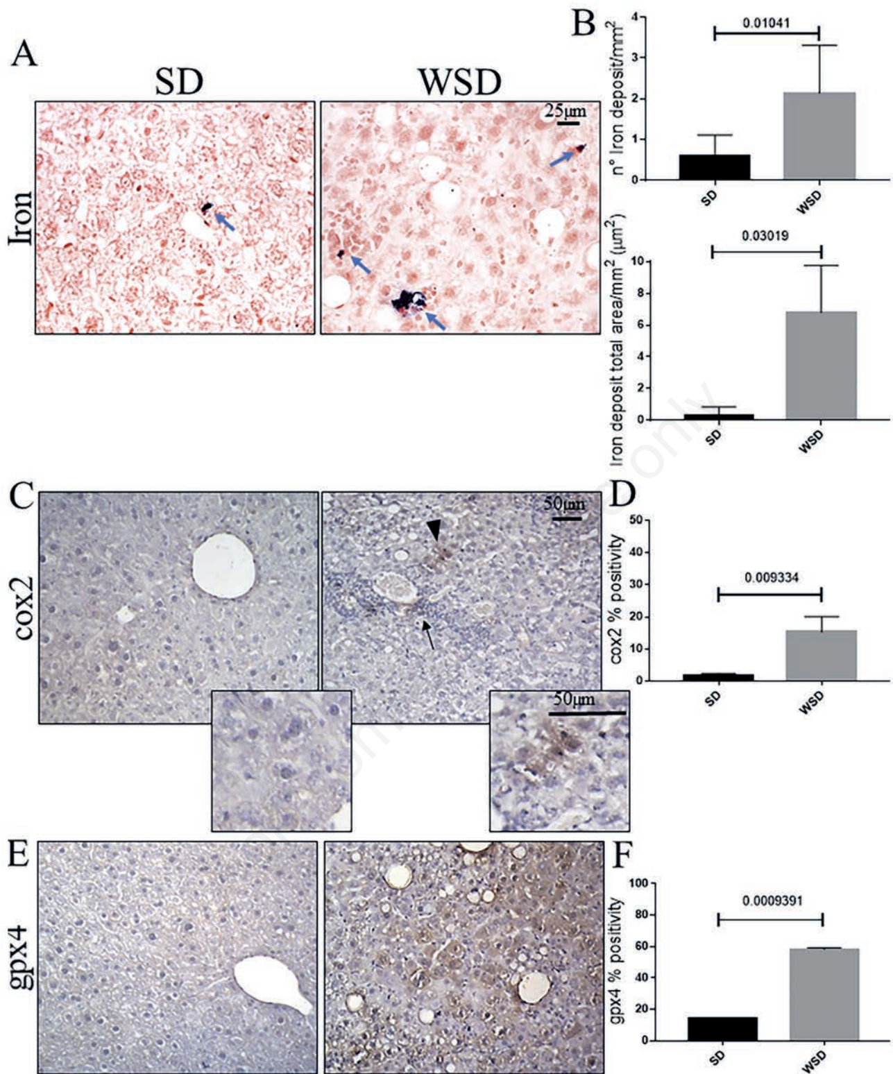
Figure 4. A) Prussian blue staining showed increased iron deposits (arrows) in WSD mice compared to the SD group; original magnification 40 \times , scale bar: 25 \mu\text{m} . B) Quantification of iron deposits, in both number and area, showed a significant increase in iron content in WSD-fed mice compared to the SD group. C) Immunohistochemistry for Cox2 showed an increase in immunopositivity in WSD compared to SD mice; original magnification 20 \times , scale bar 50 \mu\text{m} ; inset, scale bar: 50 \mu\text{m} ; arrowhead, epithelial-like Cox2-positive cells; arrow, Cox2-positive inflammation focus. D) Semi-quantitative analyses confirmed a significant increase in Cox2 expression. E) Immunohistochemistry of Gpx4 showed increased positivity in WSD mice compared to the SD group; original magnification 20 \times , scale bar: 50 \mu\text{m} . F) The semi-quantitative evaluation highlighted a significant increase of expression in WSD-fed mice compared to the SD group. These images are representative of n=8 SD, and n=8 WSD mice. Values represent means \pm standard deviation. Data were analyzed using the Mann-Whitney test; SD, standard diet; WSD, Western-style diet.
